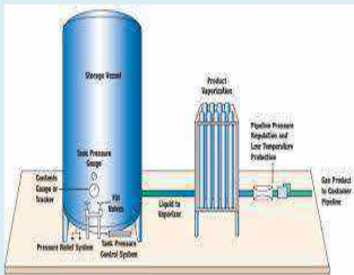
Liquid Nitrogen Vaporizer
